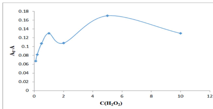
Fig. 3 Effect of H_2O_2 on the generation of hydroxyl radicals from samples containing 3 mL of 1.5 \times 10^{-4} mmol 4, 3.375 \times 10^{-5} mmol methylene blue and H_2O_2 at different concentrations. Reproduced with permission from Li et al. , 2019. Copyright 2019, Royal Society of Chemistry.
