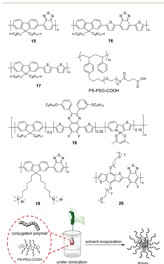
Fig. 6 Chemical structures of polymers 15–20 and preparation of polymer dots (Pdots) by the nano-precipitation method for photocatalytic \text{H}_2 production. The scheme is adapted with permission from ref. 82, Copyright 2016 Wiley-VCH.
