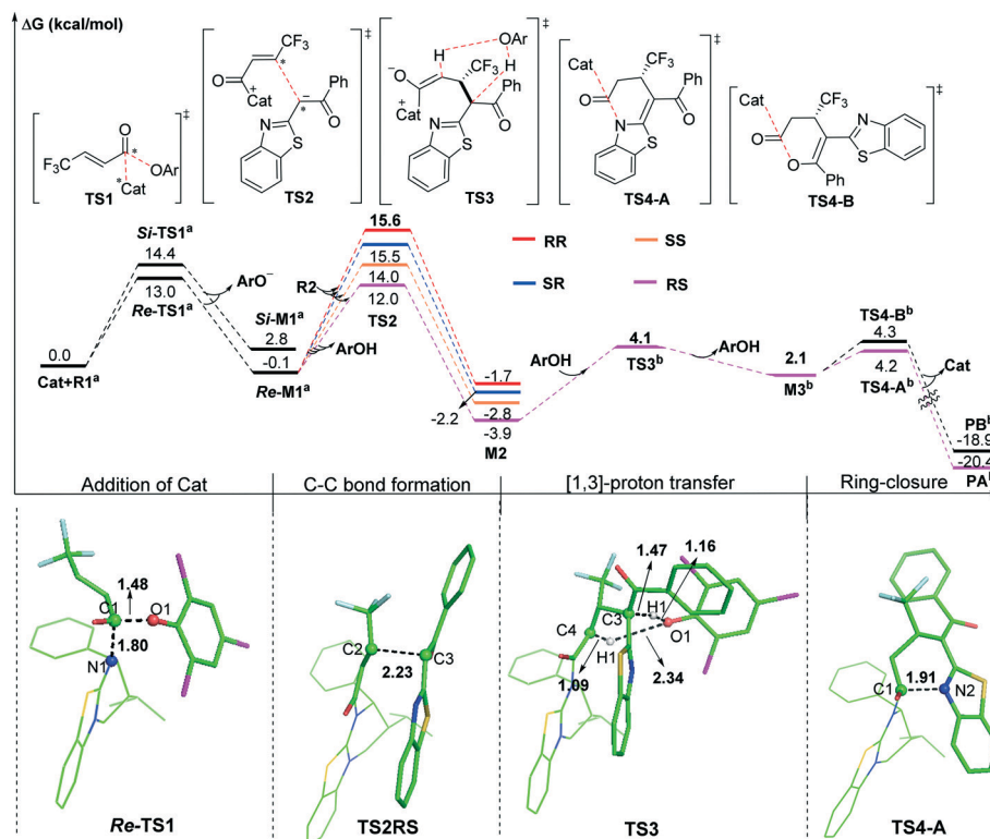
Fig. 1 The relative Gibbs free energy profiles of the isothiurea-catalyzed [3 + 3] annulation reaction. (the superscript “ a ” represents adding the free energy of pre-R2, the superscript “ b ” represents the S configuration, and distances are in angstroms).
