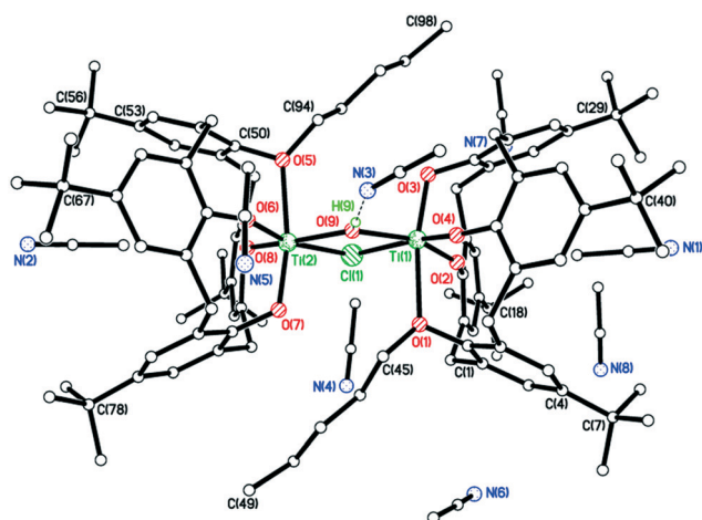
Fig. 5 Molecular structure of \{[\text{Ti}(\text{O})_3(\text{On-penty})]_2(\mu\text{-Cl})(\mu\text{-OH})\cdot 7.5\text{MeCN} (7.5MeCN) (most H atoms are omitted for clarity). Selected bond lengths (Å) and angles ( ^\circ ): Ti(1)–O(1) 2.342(2), Ti(1)–O(2) 1.815(2), Ti(1)–O(3) 1.880(2), Ti(1)–O(4) 1.786(2), Ti(1)–O(9) 1.991(2), Ti(1)–Cl(1) 2.5128(8), O(1)–Ti(1)–O(3) 169.08(8), O(2)–Ti(1)–O(4) 104.48(9), Cl(1)–Ti(1)–O(9) 74.02(6), Ti(1)–O(1)–C(1) 114.29(16), Ti(1)–O(2)–C(12) 149.03(17), Ti(1)–O(3)–C(23) 119.70(17), Ti(1)–O(4)–C(34) 165.2(2).
