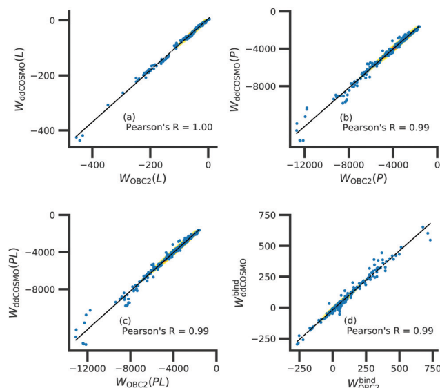
Fig. 10 Comparison of solvation free energy estimates (in \text{kcal mol}^{-1} ) based on OBC2 (x-axis) and ddCOSMO (y-axis). Solvation free energy estimates are of the (a) ligand, (b) protein, (c) complex, and (d) the binding energy.
