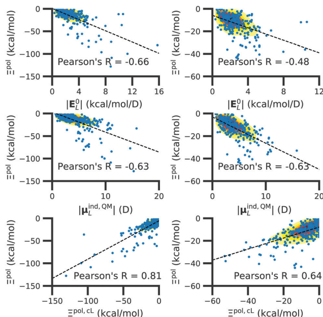
Fig. 6 The ligand polarization energy, \varepsilon^{\text{pol}} , as a function of the magnitude of the electric field |E_L^0| (top), the magnitude of the induced dipole moment |\mu_L^{\text{ind,QM}}| (middle), and the classical polarization energy \varepsilon^{\text{pol,CL}} (bottom), where E_L^0 , \mu_L^{\text{ind,QM}} , and \varepsilon^{\text{pol,CL}} are from eqn (29), (30), and (28), respectively. The range of \varepsilon^{\text{pol}} is either \varepsilon^{\text{pol}} < 0 kcal mol ^{-1} (left) or -50 kcal mol ^{-1} < \varepsilon^{\text{pol}} < 0 kcal mol ^{-1} (right).
