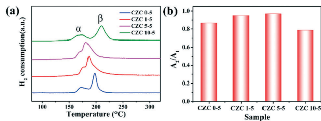
Fig. 6 (a) \text{H}_2 -TPR profiles and (b) cumulative \text{H}_2 uptake of the different CZC samples.
