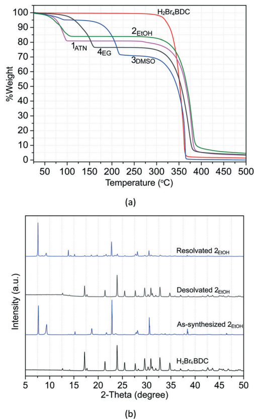
Fig. 5 TG curves of H 2 Br 4 BDC and all the solvates (a) and PXRD patterns (bottom to top) of H 2 Br 4 BDC, as synthesized 2 EIOH , desolvated 2 EIOH , and resolved 2 EIOH (b).
