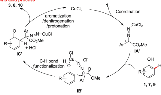
Scheme 6 Proposed catalytic cycle.
