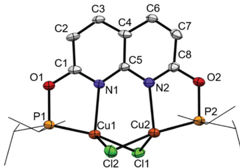
Fig. 1 Displacement ellipsoid plot (50% probability) of complex 1 in the crystal. Hydrogen atoms and THF solvent molecule are omitted, and i -Pr groups on P are depicted as wireframe for clarity.
