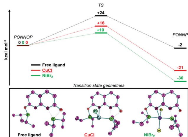
Fig. 3 DFT calculated (BP86-D3, def2-TZVP) free energy profiles ( \Delta G^{\circ}_{298K} in kcal mol –1 ) for the rearrangement of PONNOP to PONNP (top) and the transition state geometries (bottom).
