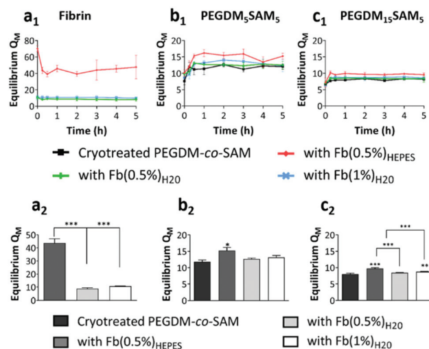
Fig. 3 Swelling characteristics of the various (a) fibrin formulations and (b) and (c) cryotreated PEGDM-co-SAM: swelling kinetics for (a 1 ) fibrin hydrogels and across fibrin-free and fibrin-containing PEGDM-co-SAM hydrogels: (b 1 ) PEGDM 5 SAM 5 and (c 1 ) PEGDM 15 SAM 5 . Swelling mass ratio ( Q_M ) at equilibrium for (a 2 ) fibrin hydrogels and across fibrin-free and fibrin-containing PEGDM-co-SAM hydrogels: (b 2 ) PEGDM 5 SAM 5 and (c 2 ) PEGDM 15 SAM 5 . The swelling ratios Q_M at equilibrium measured on the different fibrin-containing PEGDM-co-SAM hydrogels were compared to those of fibrin-free cryotreated PEGDM-co-SAM hydrogels and to each other. Values represent mean \pm SD ( n \geq 3 ). Data were analyzed using one-way ANOVA test. * p < 0.05 , ** p < 0.01 , and *** p < 0.001 .
