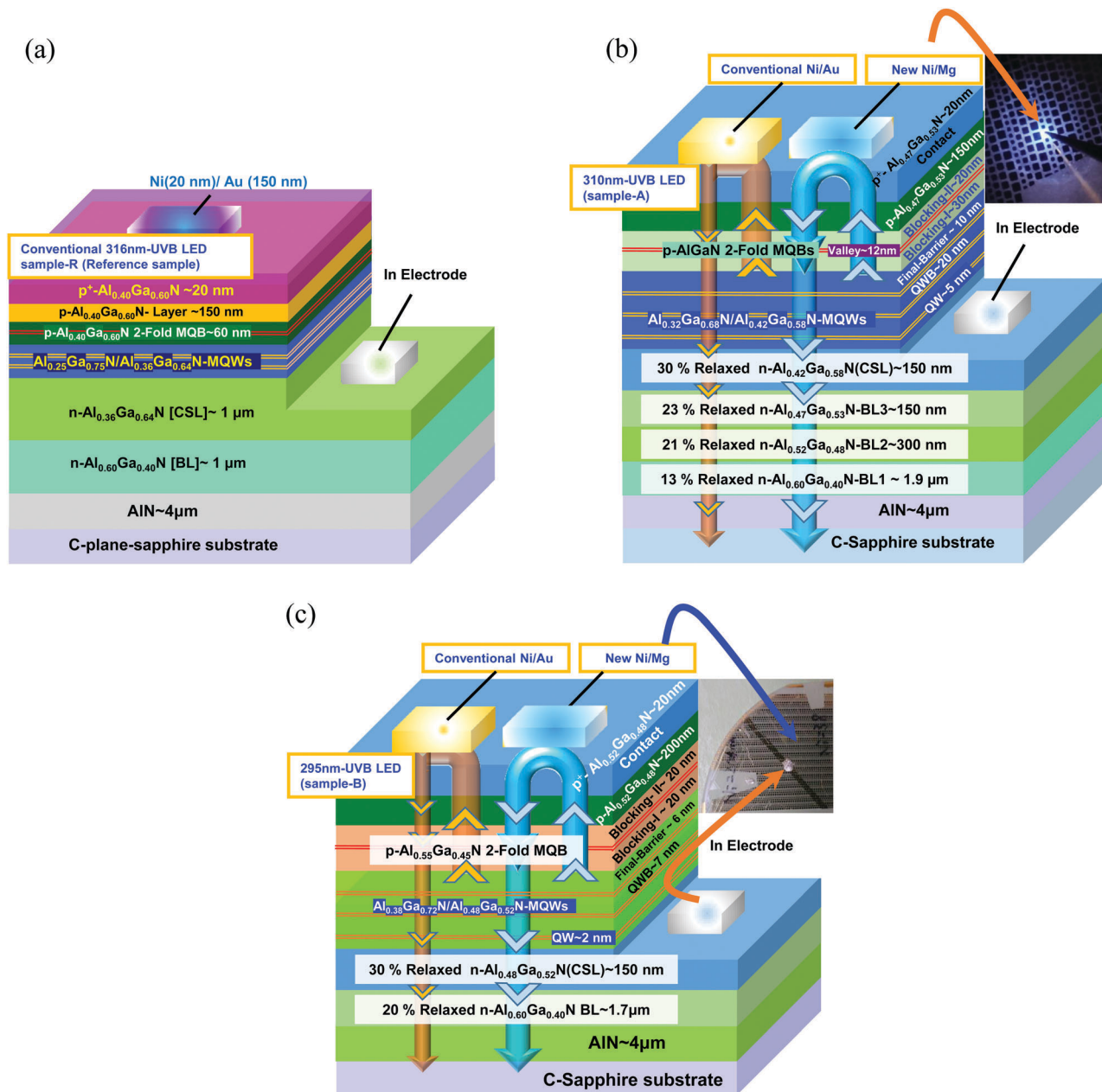
Fig. 1 (a) Schematic of 2-stack conventional AlGa 0.40 N BL based 316 nm UV-B LEDs, with a conventional Ni/Au p-electrode (sample-R), (b) schematic of 4-stack AlGa 0.47 N BL based 310 nm UV-B LEDs, one with a conventional Ni/Au p-electrode and the other one with a highly-reflective Ni/Mg p-electrode (the real image of 310 nm UV-B LED device under operation with p-electrode is shown in the inset), and (c) schematic of 2-stack AlGa 0.52 N BL based 295 nm UV-B LEDs, one with a conventional Ni/Au p-electrode and the other one with a highly-reflective Ni/Mg p-electrode (the real image of 295 nm UV-B LED with both In-dot n-electrode and p-electrode is shown in the inset).
