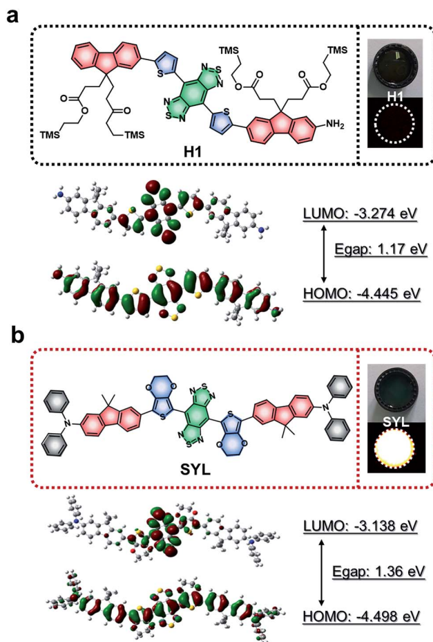
Fig. 2 Chemical structures and electronic properties of SYL and the previously reported NIR-II dye H1 : (a) Frontier orbitals of H1 , its associated energies (DFT using B3LYP Gaussian 09), and NIR-II fluorescence signals. (b) Chemical structures, NIR-II fluorescence signals and Frontier orbitals with associated energies of the novel NIR-II dye SYL .
