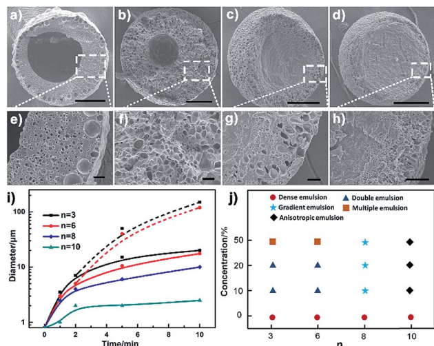
Fig. 4 SEM images of polymerized emulsions after 10 minutes of phase separation by using the C_n\text{vim}[\text{Tf}_2\text{N}]\text{-LiTf}_2\text{N} (1 : 1/5) mixture, n = 3 (a and e), n = 6 (b and f), n = 8 (c and g) and n = 10 (d and h). (i) Average pore diameter during the phase separation process by using the C_n\text{vim}[\text{Tf}_2\text{N}]\text{-LiTf}_2\text{N} (1 : 1/5) mixture (solid line: shell pore diameter, dashed line: core diameter) and (j) morphology diagram of polymerized complex emulsions induced by using ILs containing different \text{LiTf}_2\text{N} amounts. Scale bars are 150\ \mu\text{m} (a–d) and 20\ \mu\text{m} (e–h).
