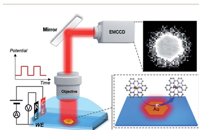
Scheme 1 Schematic illustration of ECL imaging of electrocatalytic activity on single 2D nanocatalysts. ITO as the working electrode (WE), Ag/AgCl as the reference electrode (RE) and Pt wire as the counter electrode (CE) were used.
