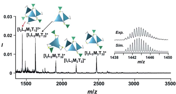
Fig. 6 Positive ESI-MS spectrum of \text{Im}_3^{\text{S}_3}\text{Bz} (normalized by its most intense fragment at m/z = 564.3 from the free ligand) in acetonitrile ( 2.2 \times 10^{-3} M) in the presence of \text{Zn}^{2+} ( 1.7 \times 10^{-3} M) and \text{ImH}_2 ( 1.7 \times 10^{-3} M). Inset: isotopically resolved signals at m/z = 1440.5 and calculated isotopic distributions for [(\text{ImH})_3(\text{Im}_3^{\text{S}_3}\text{Bz})_4(\text{Zn}^{2+})_3(\text{OSO}_2\text{CF}_3)(\text{CH}_3\text{CN})_2]^{2+} . Objects correspond to the mass peak assignment (I: \text{ImH}^+ , L: \text{Im}_3^{\text{S}_3}\text{Bz} , M: \text{Zn}^{2+} , T: \text{OSO}_2\text{-CF}_3^- ). Mass spectrum of the whole region is given in Fig. S9†
