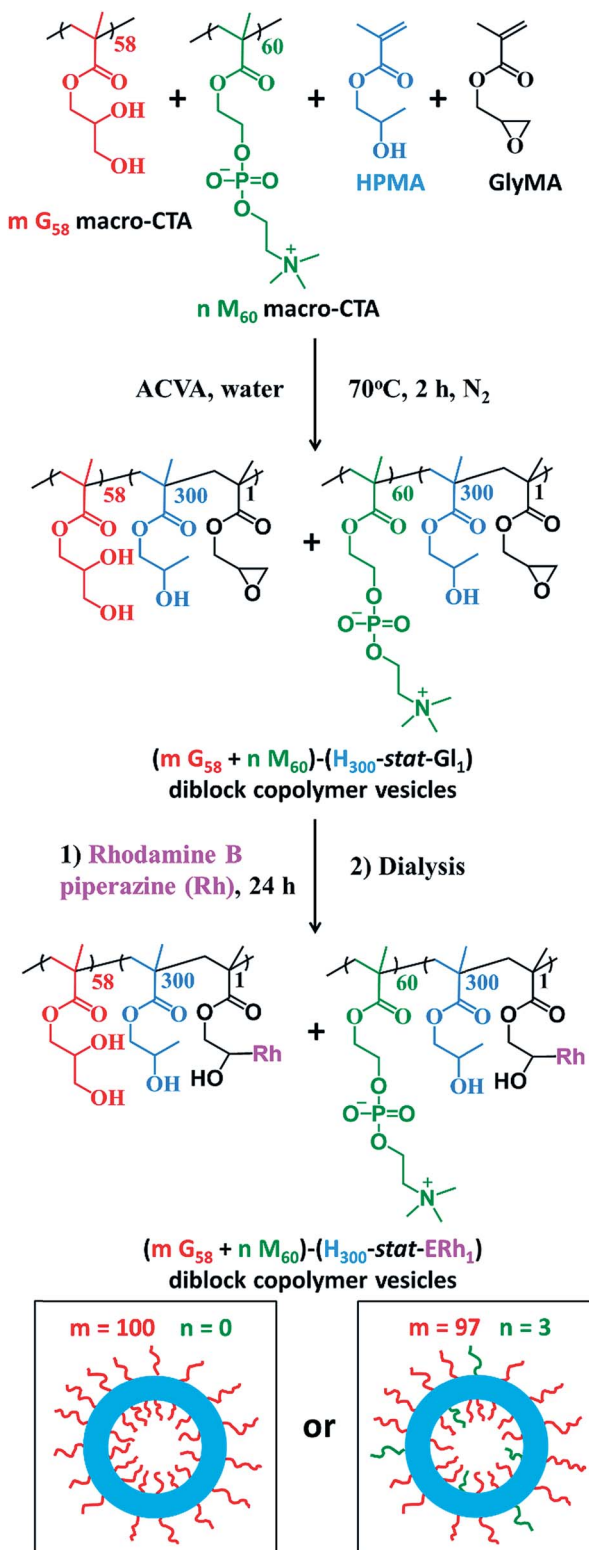
Fig. 1 Synthesis of fluorescently-labelled PGMA_{58} - P(HPMA_{300}\text{-stat-GlyMARh}_1) diblock copolymer vesicles (denoted G_{58}\text{-(H}_{300}\text{-stat-ERh}_1) , where m = 100 and n = 0 ) and (97 PGMA_{58} + 3 PMPC_{60})\text{-P(HPMA}_{300}\text{-stat-GlyMARh}_1) diblock copolymer vesicles (denoted (97 G_{58} + 3 M_{60})\text{-(H}_{300}\text{-stat-ERh}_1)\text{-D}_{52} where m = 97 and n = 3 ) via RAFT aqueous dispersion polymerization. Corresponding schematic cartoons are also shown for each type of precursor vesicle, where PGMA = red, PMPC = green, P(HPMA\text{-stat-ERh}_1) = blue. RAFT end-groups are omitted from chemical structures to aid clarity.
