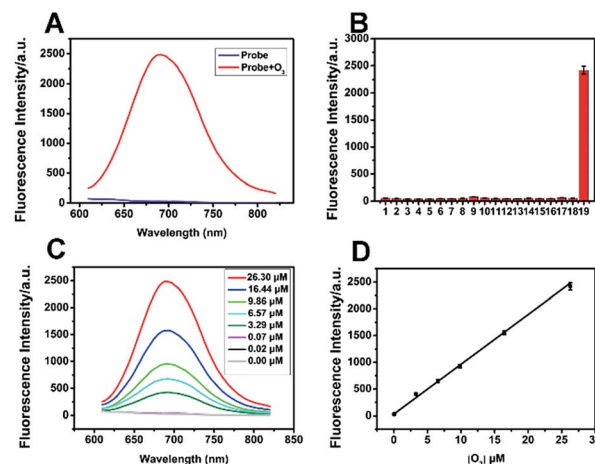
Fig. 1 Fluorescence spectral properties of ACy7. (A) Fluorescence emission spectrum of 10 \mu M ACy7 before and after reaction with O_3 (26.30 \mu M ). (B) Fluorescence responses of 10 \mu M ACy7 to some biological interfering substances. (C) Fluorescence response of 10 \mu M ACy7 after the addition of serial concentrations of O_3 . (D) A linear relationship between the fluorescence emission intensity of the ACy7 solution and the O_3 concentration ( \lambda_{ex}/\lambda_{em} = 570/690 nm). Error bars are \pm SD ( n = 3). (Interfering substances: (1) blank, (2) H_2O_2 (0.1 mM), (3) O_2^{\cdot-} (125 \mu M ), (4) ^1O_2 (50 \mu M ), (5) \cdot OH (50 \mu M ), (6) t -BuOOH (30 \mu M ), (7) NaClO (50 \mu M ), (8) NO (50 \mu M ), (9) ONOO − (6 \mu M ), (10) GSH (5 mM), (11) vitamin C (0.3 mM), (12) Na + (0.5 mM), (13) K + (0.5 mM), (14) Zn 2+ (0.5 mM), (15) Ca 2+ (0.5 mM), (16) Na 2 S 2 O 3 (0.5 mM), (17) Fe 3+ (0.5 mM), (18) citric acid (50 \mu M ), and (19) O_3 (26.30 \mu M ).)
