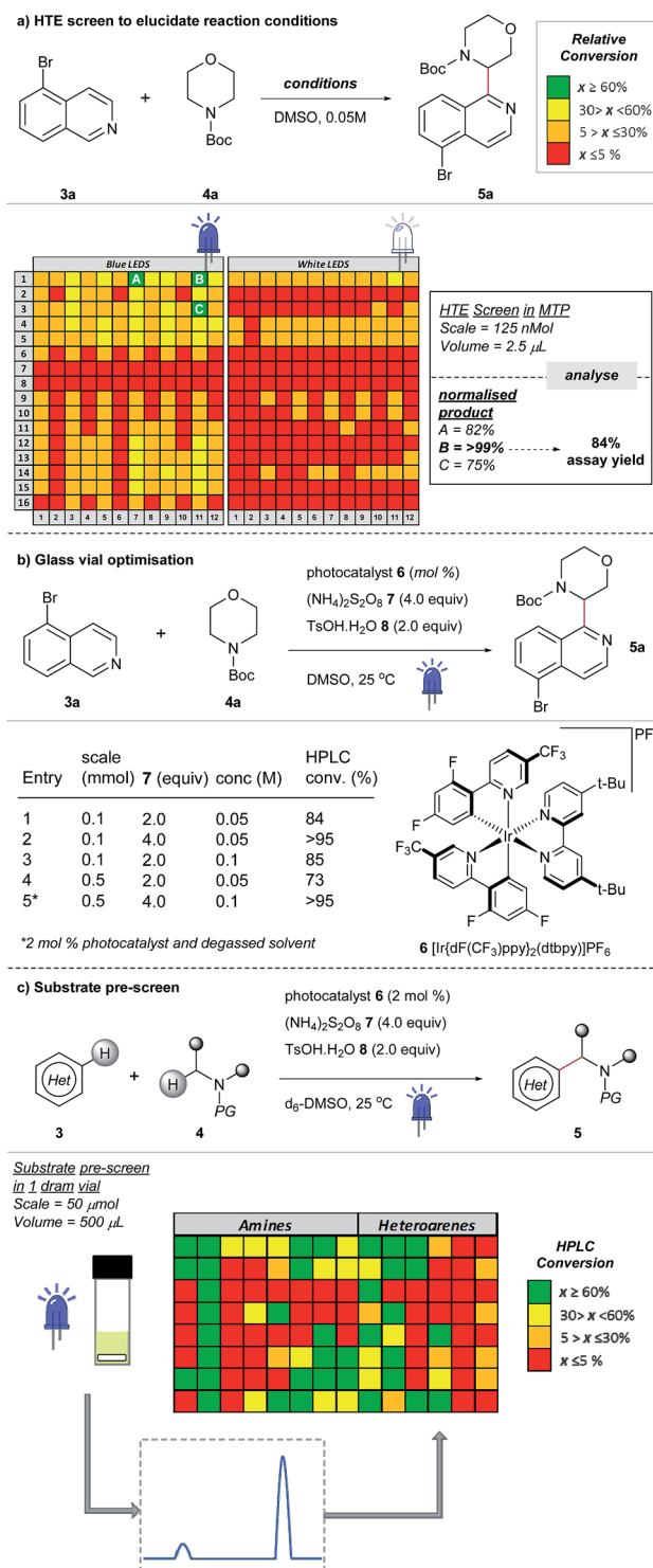
Fig. 3 Development of a new cross-dehydrogenative coupling of heteroarenes and heterocycles using an initial nanomolar HTE screen in a 1536-well MTP.
