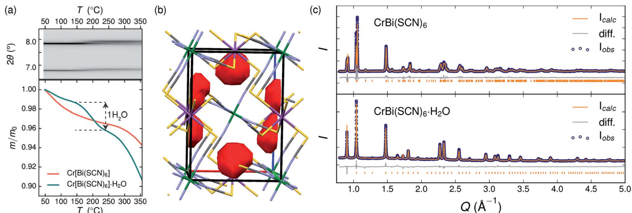
Fig. 3 (a) Dehydration of \text{Cr}[\text{Bi}(\text{SCN})_6] \cdot \text{H}_2\text{O} between 150 °C and 200 °C. Top panel: variable temperature PXR measurements of \text{Cr}[\text{Bi}(\text{SCN})_6] \cdot \text{H}_2\text{O} , highlighting the separation of the \{110\} and \{002\} reflections at around 2\theta = 7.8^\circ . Bottom panel: TGA measurements on hydrated (teal) and anhydrous (orange) show the presence of a step at around 170 °C in the hydrated sample, but no similar step in the dehydrated sample. (b) Structure of \text{Cr}[\text{Bi}(\text{SCN})_6] \cdot \text{H}_2\text{O} determined from powder diffraction data, with guests removed. The void space within the cell is shown in red (contact surface determined using Mercury, probe size 1.2 Å). Colour scheme as follows: Bi, purple; Cr, green; N, blue; C, black and S, yellow. (c) Rietveld refinement of synchrotron powder diffraction data for both hydrated and anhydrous \text{Cr}[\text{Bi}(\text{SCN})_6] .
