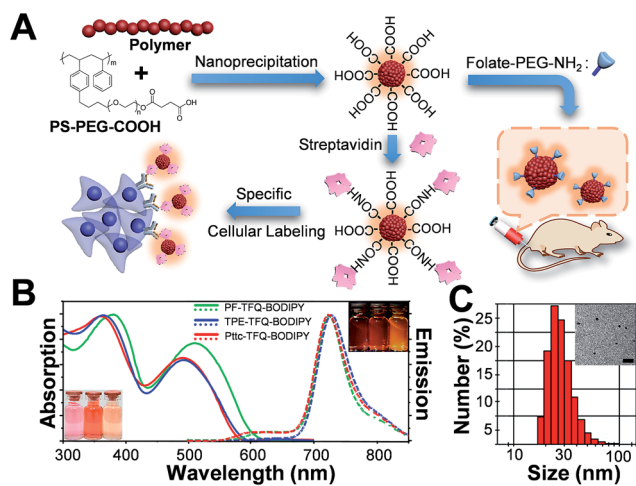
Fig. 1 (A) Schematic illustration of the preparation of carboxyl-functionalized Pdots through nanoprecipitation and subsequent bioconjugation for in vitro specific cellular imaging and in vivo tumor targeting. (B) Absorption spectra of PF-TFQ-BODIPY Pdots (solid green line), TPE-TFQ-BODIPY Pdots (solid blue line), and Pttc-TFQ-BODIPY (solid red line) in water. Their corresponding emission spectra are shown with dashed lines. The insets in the bottom-left and upper-right corners show the photographs of the Pdot solutions (from left to right: PF-TFQ-BODIPY, TPE-TFQ-BODIPY, and Pttc-TFQ-BODIPY Pdots) under daylight and under UV light illumination, respectively. (C) Hydrodynamic diameters of Pttc-TFQ-BODIPY Pdots measured by dynamic light scattering. The inset shows the transmission electron microscopy image of Pttc-TFQ-BODIPY Pdots. Scale bar is 100 nm.
