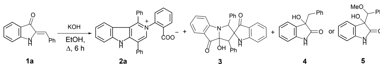
Scheme 1 Transformation of hemiindigo 1a in the alkaline conditions.
