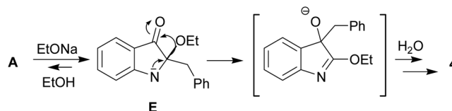
Scheme 4 Proposed route for the aza-benzilic type rearrangement of indoleninone A into 4 .
