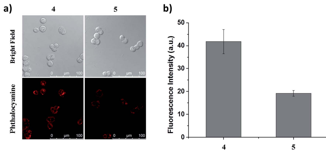
Fig. 4 (a) Bright-field and fluorescence images of HT29 cells after incubation with conjugate 4 or 5 (2 µM) for 10 min, followed by incubation in a drug-free medium for 6 h. (b) The corresponding quantified fluorescence intensities. Data are expressed as the mean \pm standard error of the mean (SEM) of three independent experiments.
