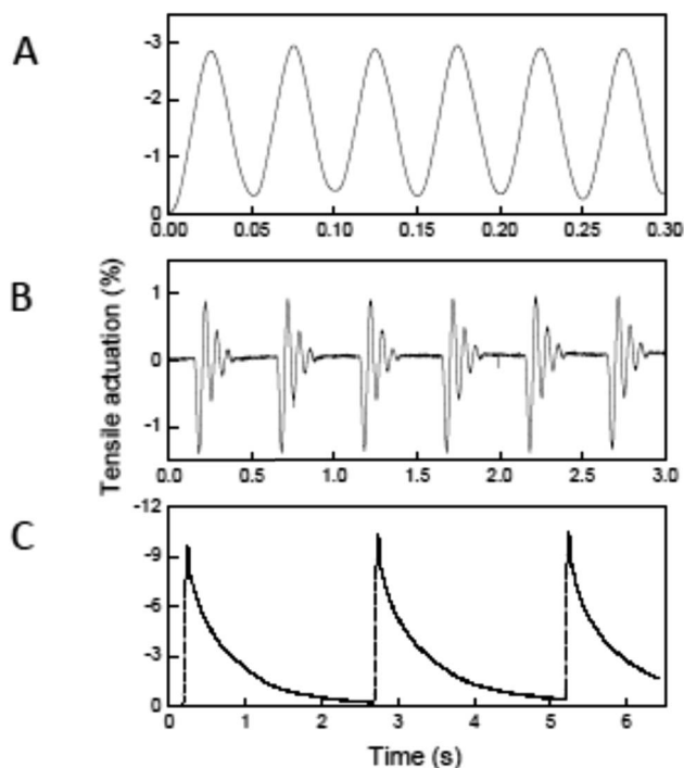
Fig. 12 Electro-thermal tensile actuation for two-end-tethered, wax-filled MWNT yarns. (A) Tensile actuation strain versus time after 1 400 000 reversible cycles for a 11.5\ \mu\text{m} diameter, coiled yarn having \sim 25\ 000 turns per m twist when driven by a 18.3\ \text{V cm}^{-1} , 20 Hz symmetric square wave voltage while lifting a load that provided a 14.3 MPa stress. (B) Tensile actuation for the yarn of (A) with 109 MPa applied tensile stress when driven at a 3% duty cycle by 15 ms, 32\ \text{V cm}^{-1} square-wave voltage pulses having a period of 500 ms. (C) Tensile strain versus time for a 150\ \mu\text{m} diameter coiled yarn when supporting a 5.5 MPa tensile stress and driven by a 15\ \text{V cm}^{-1} square wave having a 50 ms pulse duration and 2.5 s period. This figure has been reproduced from ref. 4 with permission from AAAS.
