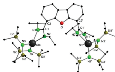
Fig. 1 Molecular structure of 1 in the solid-state. Hydrogen atoms are omitted for clarity. Selected bond lengths [Å]: Sm-Sm' 8.884, Sm-N1 2.37(2), Sm-N2 2.42(2), Sm-N3 2.282(14), Sm-N4 2.30(2), Si1-N3 1.73(2), Si2-N3 1.70(2), Si3-N4 1.68(2), Si4-N4 1.71(2), N1-C1 1.35(2), N2-C1 1.29(2); N1-Sm-N2 55.4(6), N2-C1-N1 115.0(2), N3-Sm-N4 136.0(5).
