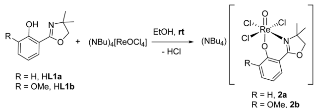
Scheme 3 Synthesis of (NBu 4 ) [ReOCl 3 ( L1a–b )] 2a–b .
