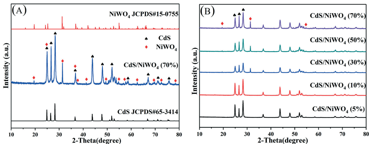
Fig. 1 The XRD patterns of (A) \text{CdS}/\text{NiWO}_4 \text{ (70\%)} and JCPDS of CdS and \text{NiWO}_4 ; (B) the XRD patterns of [\text{CdS}/\text{NiWO}_4 \text{ (} x\% \text{)}] ( x = 5, 10, 30, 50, 70 ).
