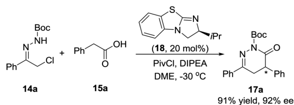
Scheme 7 Isothioureia catalyzed formal [4+2] cycloaddition of azoalkenes with arylacetic acids and the proposed mechanism.
