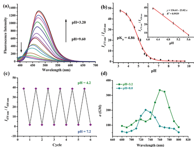
Fig. 1 (a) Emission spectra of Lyso-MPCB (10 \mu\text{M} ) in B–R buffer solution with different pH from 9.60 to 3.20 (with 30% DMSO, \lambda_{\text{ex}} = 370 \text{ nm} ). (b) Plot of the fluorescence intensity ratio ( I_{475\text{nm}}/I_{410\text{nm}} ) vs. pH. Inset: Linear relationship of pH-dependent fluorescence intensity ratio ( I_{475\text{nm}}/I_{410\text{nm}} ). R^2 = 0.9939 . (c) pH reversibility of Lyso-MPCB in B–R buffer solution (pH = 4.20 and 7.20). (d) Two-photon absorption cross-section of Lyso-MPCB with pH = 3.2 and 8.0, respectively. ( \lambda_{\text{ex}} = 680\text{--}800 \text{ nm} ).
