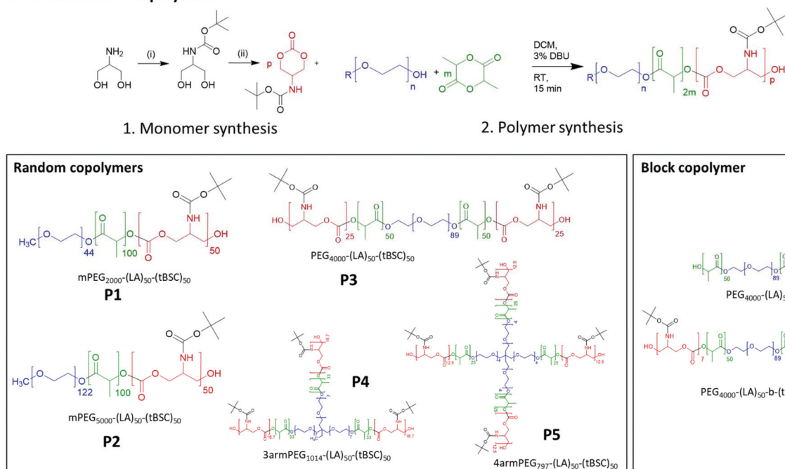
Scheme 1 Synthesis of monomer and PEG-initiated copolymers of varying architectures and block compositions.
