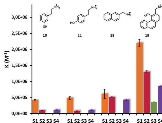
Fig. 7 Graphical representation of binding constants of analytes 10, 11, 18, 19 and S1 -, S2 -, S3 - and S4 -AuNPs. Values of association constants and binding sites with their uncertainties are reported in Table S1 in the ESI.†
