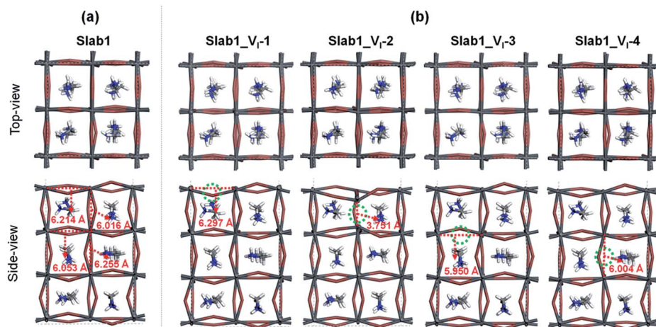
Fig. 2 (a) Defect-free and (b) V I -containing defective MAPbI 3 slabs. The dashed circles indicate the position of the V I . Each number in (b) indicates the Pb–Pb distance around the V I .
