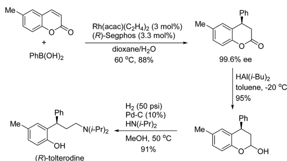
Scheme 3 The enantioselective 1,4-addition of arylboronic acids to \beta -aryl substituted unsaturated carbonyl derivatives.
