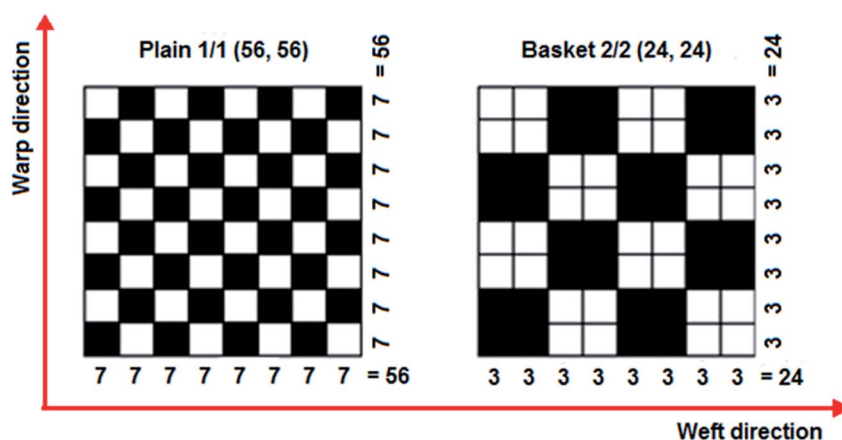
Fig. 1 Schematic views of interlacement placement in the p -aramid fabrics (plain 1/1 and basket 2/2 weaves) and number of yarn interacements in each fabric direction.
