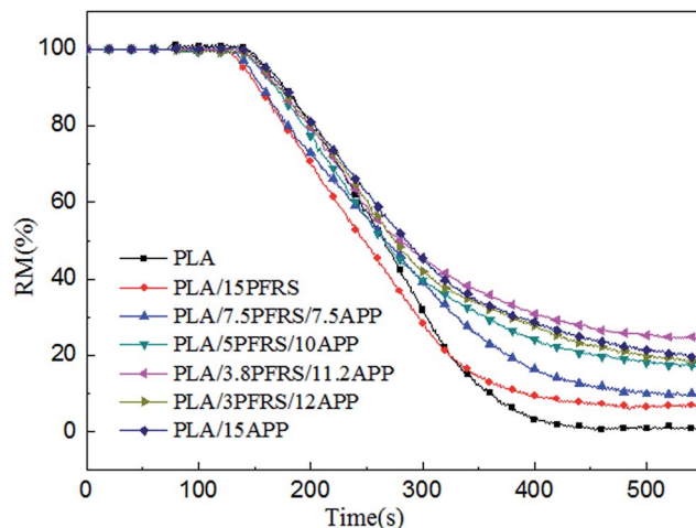
Fig. 7 Mass loss curves of pure PLA and its composites.
