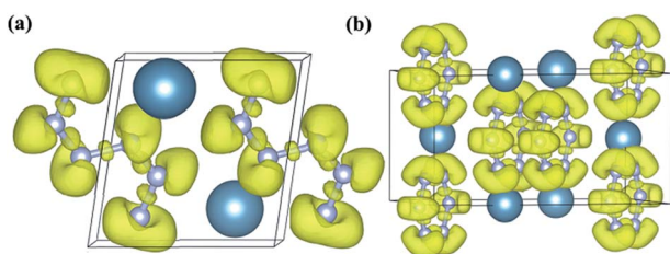
Fig. 5 The ELF distributions of (a) P\bar{1} -CaN 3 at ambient pressure and (b) C2/m -CaN 3 at 60 GPa. The value of isosurface is 0.75.
