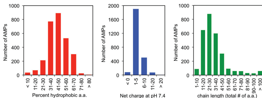
Fig. 2 Despite their lack of conserved sequence or secondary structure, there are three common physiochemical characteristics of antimicrobial peptides: (a) hydrophobicity, (b) cationic charge, and (c) short chain length. The data were collected from The Antimicrobial Peptide Database ( http://aps.unmc.edu/AP/structure.php ).
