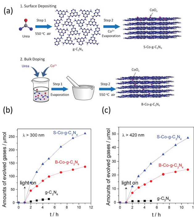
Fig. 11 (a) Schematic illustration of surface deposition and bulk doping modification of g-C_3N_4 with CoO_x . Photocatalytic water oxidation activities of the g-C_3N_4 , B-Co-g-C_3N_4 and S-Co-g-C_3N_4 samples under (b) UV ( \lambda > 300\text{ nm} ) and (c) visible light ( \lambda > 420\text{ nm} ) irradiation. Reprinted with permission from ref. 107. Copyright 2016, American Chemical Society.
