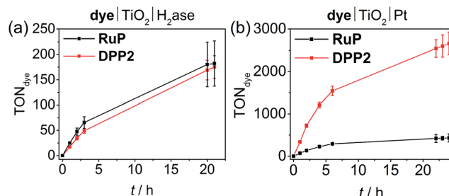
Fig. 4 (a) Photocatalytic activity of \text{DPP2}|\text{TiO}_2|\text{H}_2\text{ase} and \text{RuP}|\text{TiO}_2|\text{H}_2\text{ase} . Conditions: 2.5 mg \text{TiO}_2 , 50 pmol [\text{NiFeSe}]-\text{H}_2\text{ase} , 0.05 \mu\text{mol} of DPP2 or RuP , in 3 mL AA-MES solution (0.1 M, pH 6); (b) photocatalytic activity of \text{DPP2}|\text{TiO}_2|\text{Pt} and \text{RuP}|\text{TiO}_2|\text{Pt} . Conditions: 2.5 mg pre-platinised \text{TiO}_2 , 0.05 \mu\text{mol} of DPP2 or RuP , in 3 mL AA solution (0.1 M, pH 4.5). In both cases the samples were irradiated with UV-filtered solar light (100 \text{mW cm}^{-2} , AM 1.5G, \lambda > 420 nm) at 25 ^\circ\text{C} .
