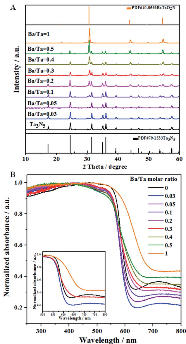
Fig. 1 Structural characterizations of typical Ba( n )-Ta 3 N 5 samples ( n = 0-1 ): (A) XRD patterns and (B) UV-vis spectra. " n " stands for the molar ratio of Ba/Ta. The inset figure is enlarged for the wavelength range of 500–800 nm.
