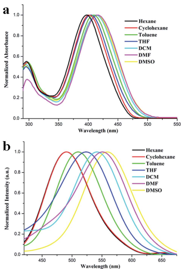
Fig. 1 Normalized UV-vis absorption (a) and fluorescent emission (b, \lambda_{\text{ex}} = 365\text{ nm} ) spectra of TBM excited at 410 nm in different solvents ( 1.0 \times 10^{-5}\text{ M} ).
