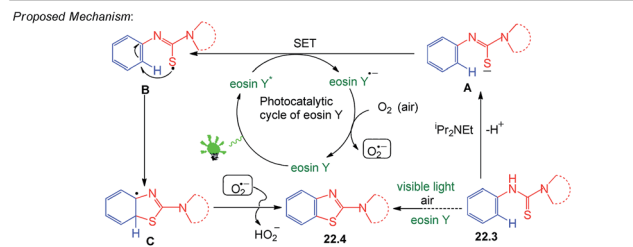
Scheme 22 Aerobic oxidative cyclization of 2-aminobenzothiazole.
