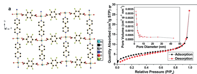
Fig. 4 (a) 2D view of Mn-LMOF. (b) N 2 adsorption–desorption isotherm of as-synthesized Mn-LMOF after grinding for 2 h, and the inset represents the pore size distribution curve.
