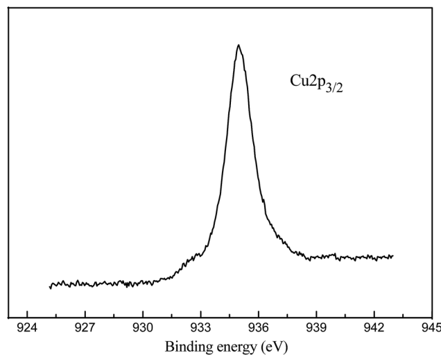
Fig. 6 XPS spectra of \text{Cu } 2p_{3/2} for FPC-1.
