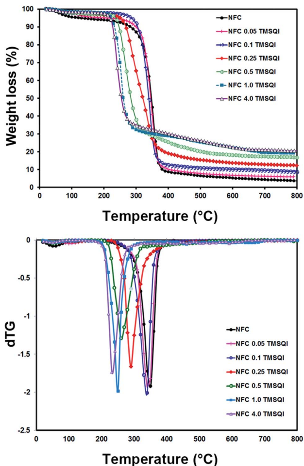
Fig. 7 TGA (a) and DTG (b) of neat NFC and NFC grafted with 0.05–4 g TMSQI.
