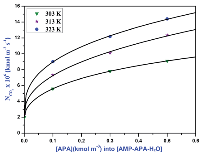
Fig. 4 Specific absorption rates of CO 2 into aqueous solutions of APA at different temperatures for gas compositions 5% CO 2 and 95% N 2 .
