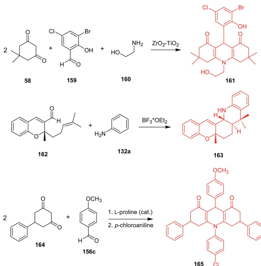
Scheme 27 Examples of newly obtained acridine derivatives 161 , 96 163 , 97,98 165 . 99
