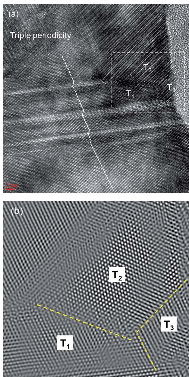
Fig. 6 (a) HRTEM micrograph corresponding to region "D" in Fig. 4. Triple periodicity and a threefold twin are observed. (b) Inverse FFT micrograph corresponding to the region indicated by the dotted square in (a).
