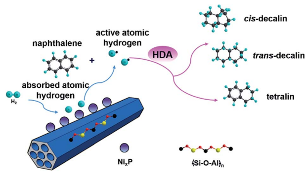
Fig. 7 Proposed reaction schematic of naphthalene HDA over highly active \text{Ni}_x\text{P} -Al-M catalyst.
