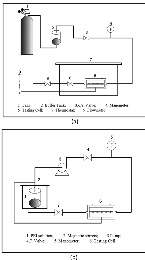
Fig. 2 Schematic diagram of the experimental setup for (a) \text{CO}_2 and \text{N}_2 permeation testing; (b) membrane preparation.
