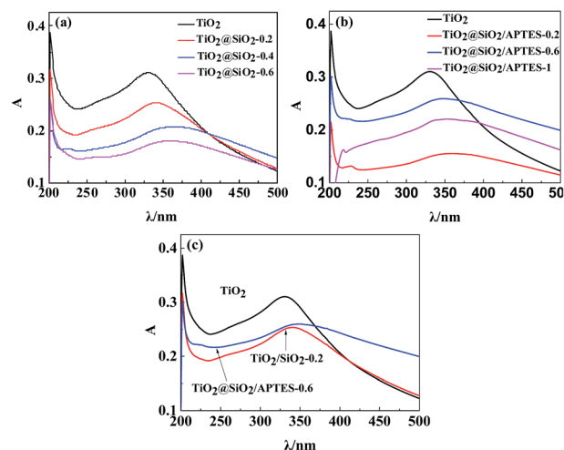
Fig. 7 UV absorbance spectra of (a) the U-TiO 2 and TiO 2 @SiO 2 (weight ratio = 0.2, 0.4, 0.6) nanoparticles, (b) the U-TiO 2 and TiO 2 @SiO 2 /APTES (weight ratio = 0.2, 0.6, 1), (c) the U-TiO 2 , TiO 2 @SiO 2 -0.2, and TiO 2 @SiO 2 /APTES-0.6 nanoparticles.
